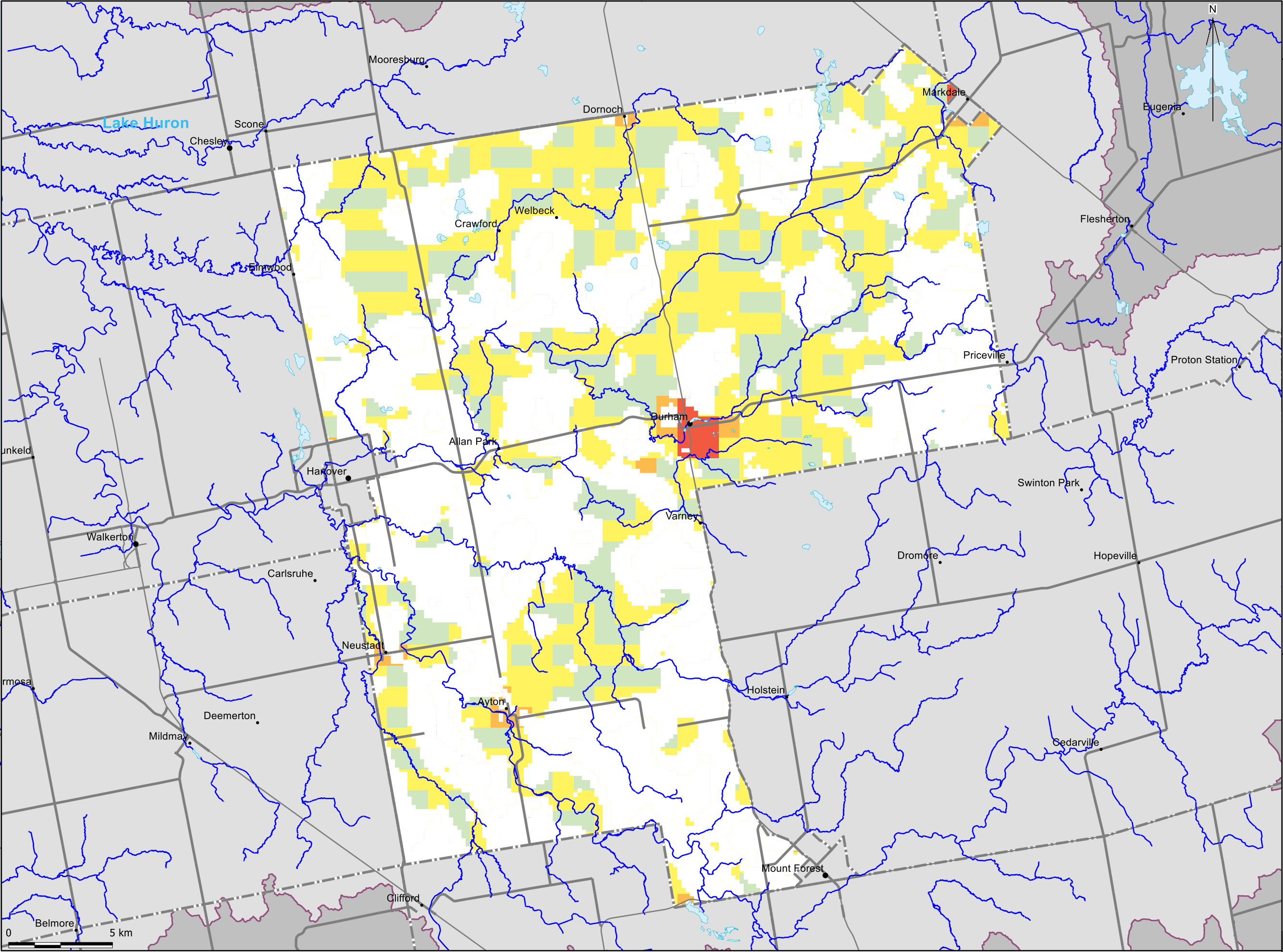
MAP 4.13.M5 IMPERVIOUS SURFACE
