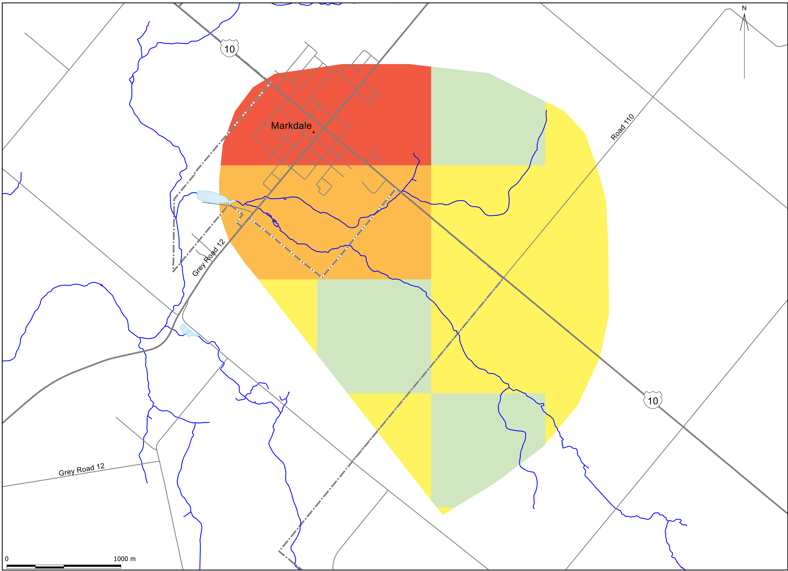
MAP 4.4.G1.4 IMPERVIOUS SURFACE - Markdale Water Quality Threats and Issues – Municipality of Grey Highlands
