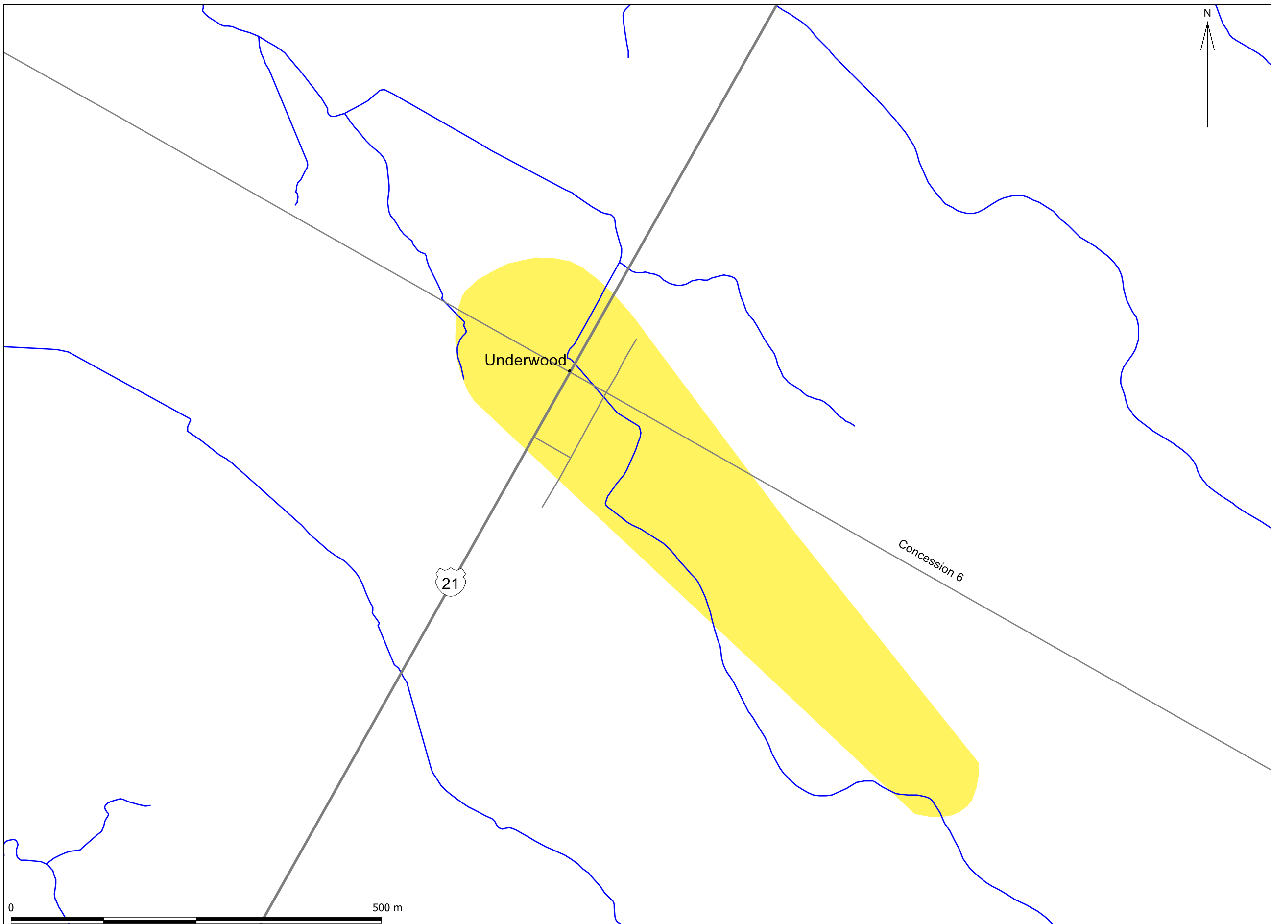
MAP 4.7.G2.4 IMPERVIOUS SURFACE - Underwood Water Quality Threats and Issues - Municipality of Kincardine
