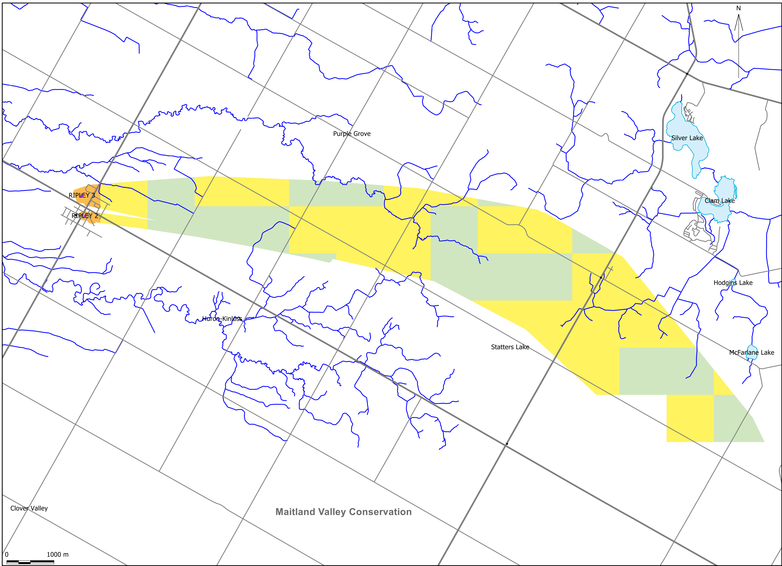
MAP 4.6.G1.4 IMPERVIOUS SURFACE, WHPA - Ripley
