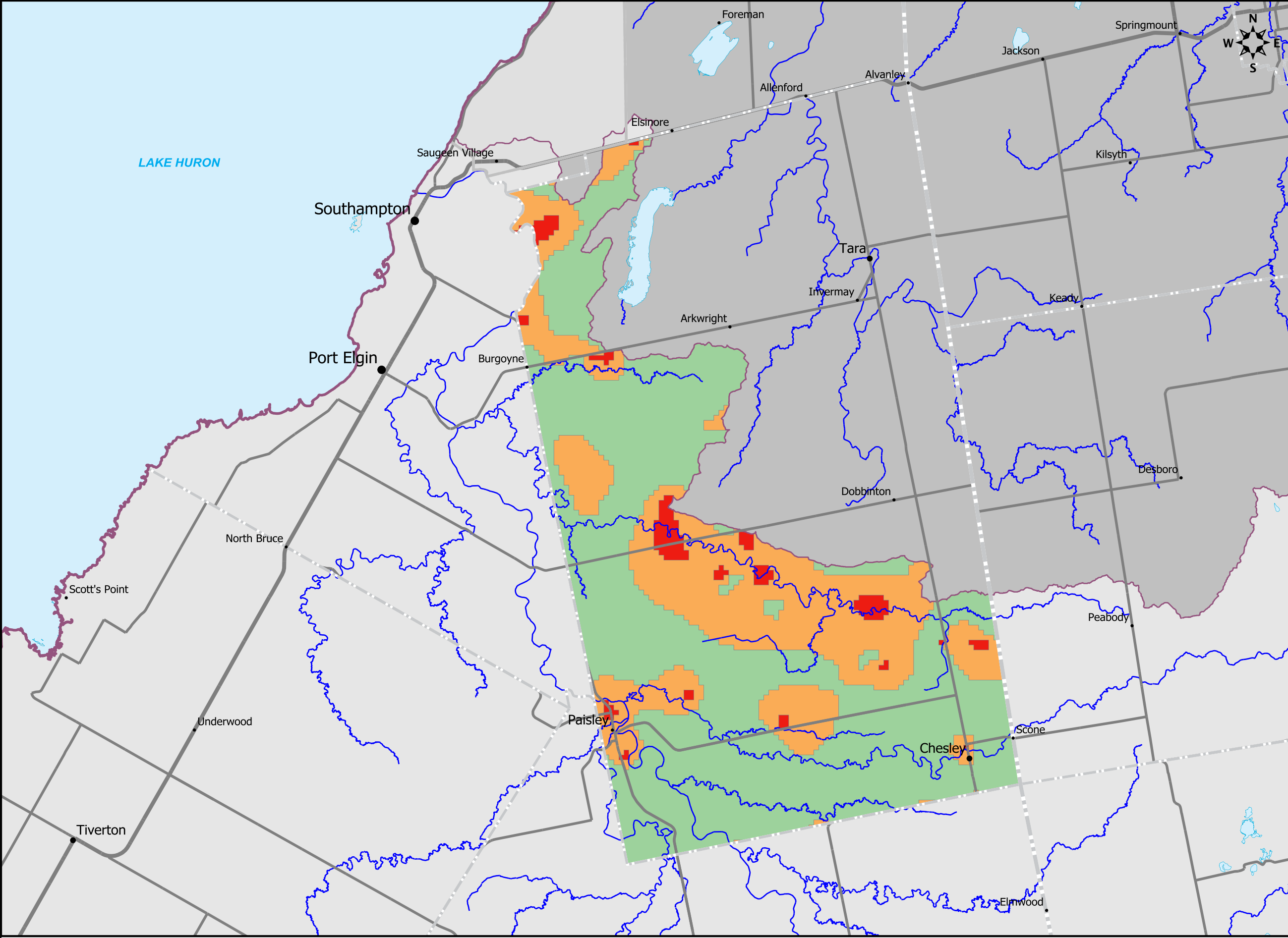
MAP 4.1.M1 INTRINSIC SUSCEPTIBILITY INDEX
