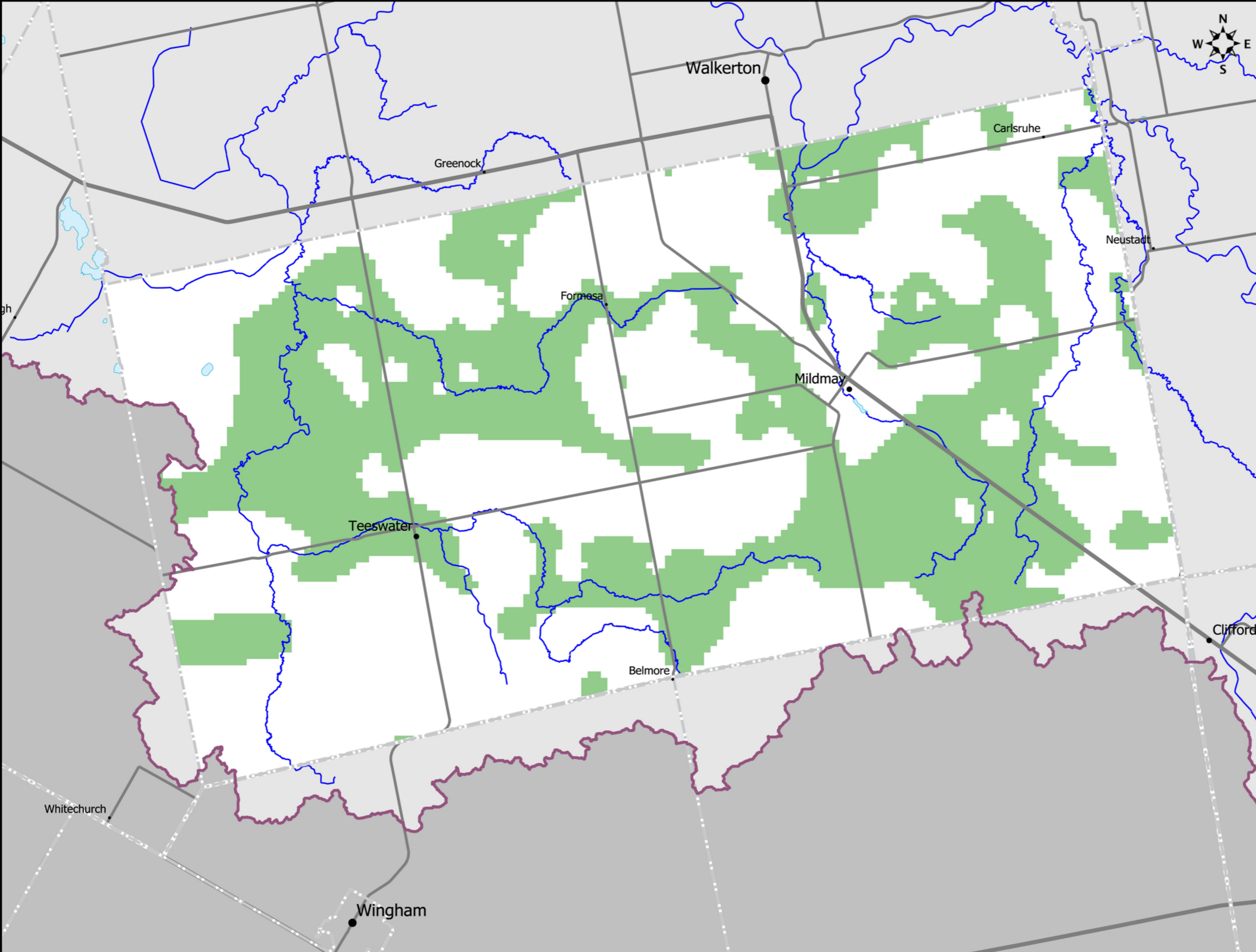
MAP 4.10.M6 HIGHLY VULNERABLE AQUIFER MANAGED LANDS
